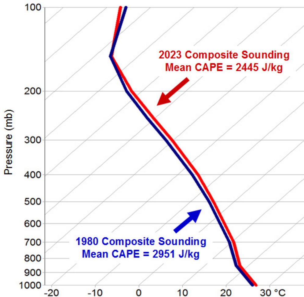
Figure 3. Pressure level temperature trend comparison and associated CAPE differences between 1980 (Blue) and 2023 (Red) composite profiles from 15 tropical island stations between 5 and 25 degrees latitude (NH: Jul-Nov, SH: Dec-Apr). Mean CAPE values are an average of three CAPE calculations: Surface based (SBCAPE), mixed layer w/25 mb depth (MLCAPE/25), and mixed layer w/50 mb depth (MLCAPE/50).
